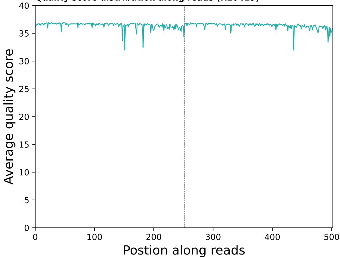
Quality score distribution along reads (R10419)
